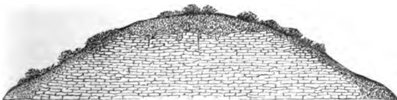
FIG. 64.—Ideal section showing result of disintegration in an unglaciated region. (Chamberlin.)
